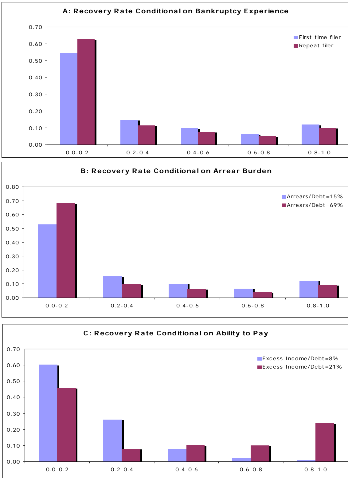
Figure 6: Model-Generated Conditional Distributions of Recovery Rates
