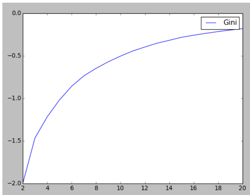
Figure 1: Gini Coefficient
