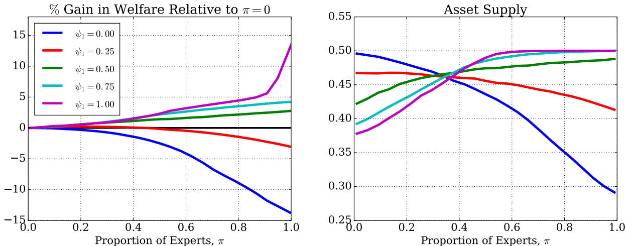
Figure 3: The effects of information on welfare and the supply of assets.
