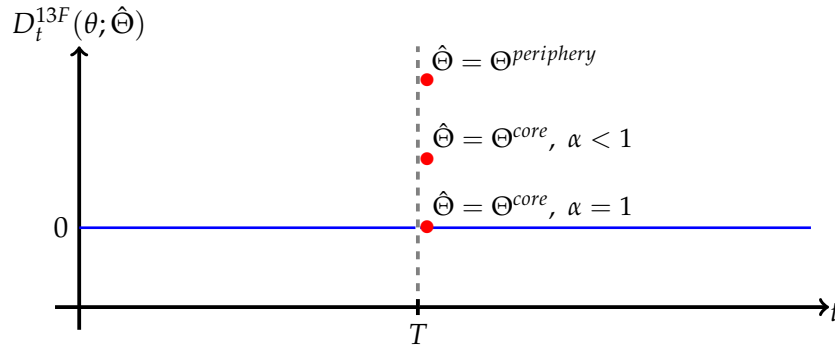
Figure 5: Filing form 13-F and the discontinuity in the probability of trade
