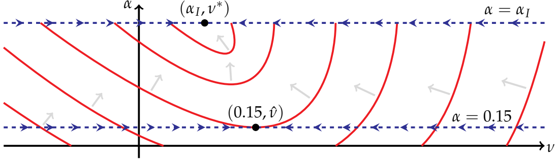
Figure 2: Trade centrality level curves
